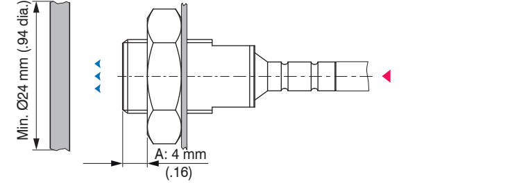
Mounting, dimensions in mm (inches, rounded off)
