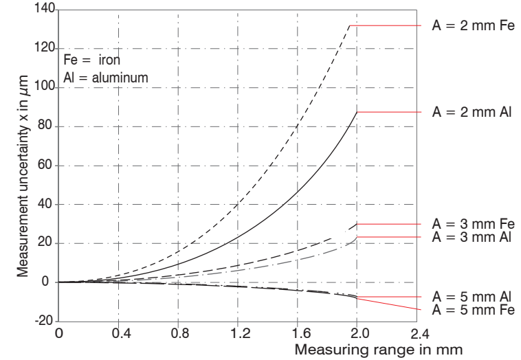
Measurement uncertainty depending on distance A and target material
