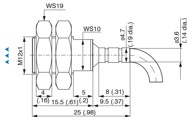
ES-S2-C-CAX, dimensions in mm (inches, rounded off)
