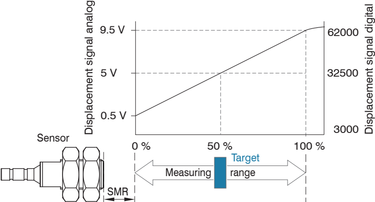
Start of measuring range (SMR), the shortest distance between the front surface of the sensor and the target.
