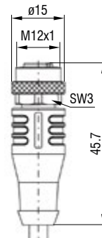
Socket PC5/5
