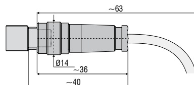
Female connector dimensions apply for all models
