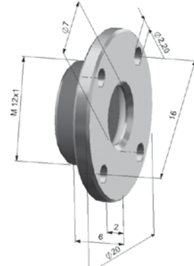
TM-CF-CX Ancillary CF lens, TM-PW-CX Protective window
