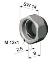
TM-CF-CS Ancillary CF lens (only for LT models)
