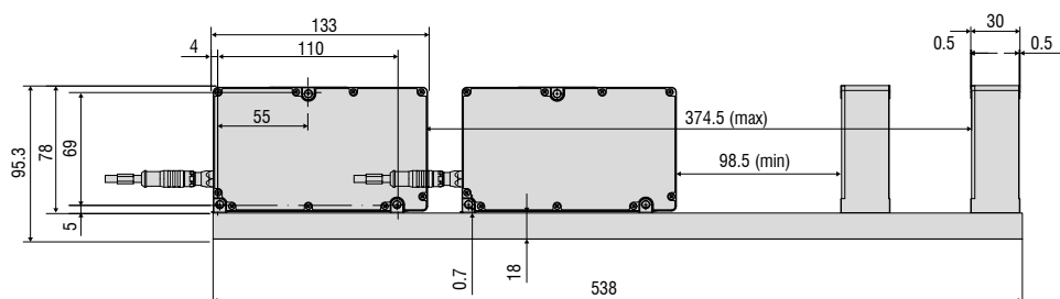
Light source and receiver with mounting rail
