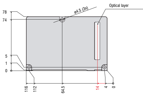
Light source
