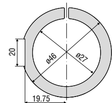
MA 2400-27 for sensors IFS2405-0,3 / -1 IFS2406-3 / -10 IFD2411-x IFD2410-x IFD2415-1
