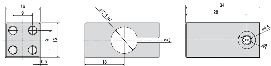
Accessories: mounting adapter
