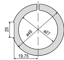
MA 2400-27 for sensors IFS2405-0,3 / -1 IFS2406-3 / -10
