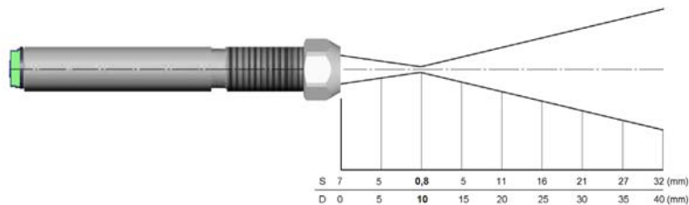
Fig. 2 Optical chart (15:1) with CF-lens (0.8 mm@ 10 mm)
