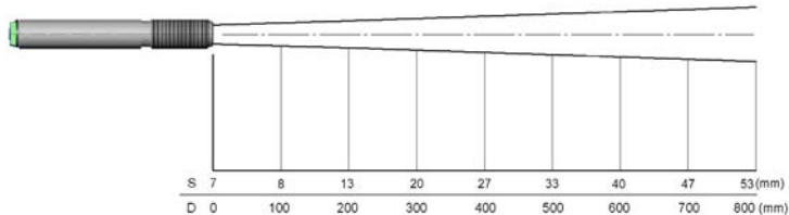
Fig. 1 Optical chart (15:1)
