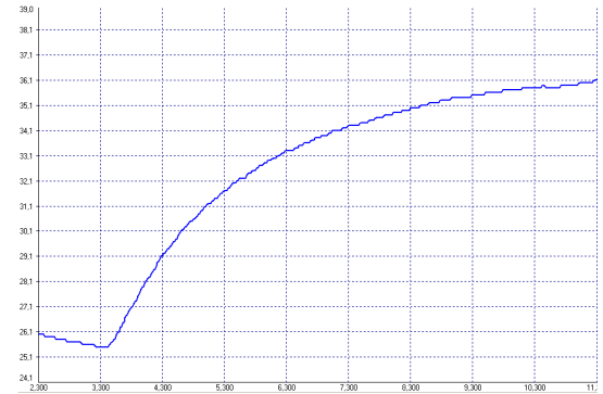
Fig. 18 Signal graph without Smart Averaging function
