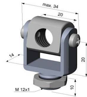
Fig. 8 Mounting fork with M12x1 thread, adjustable in two axes [TM-MG-CS]
