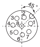
Fig. 3 View of solder pin side, 8-pin, A-coded, female connector
