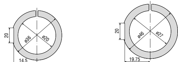
Mounting ring
