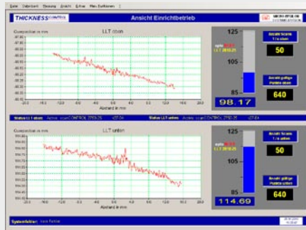
By means of the laser line triangulation, tiltings, distortions and bendings are reliable compensated.
