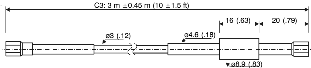
Sensor cable, Type C3
